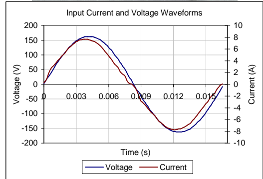
Input AC Current Waveform (ITHD = 6.87%, 50% Load)
